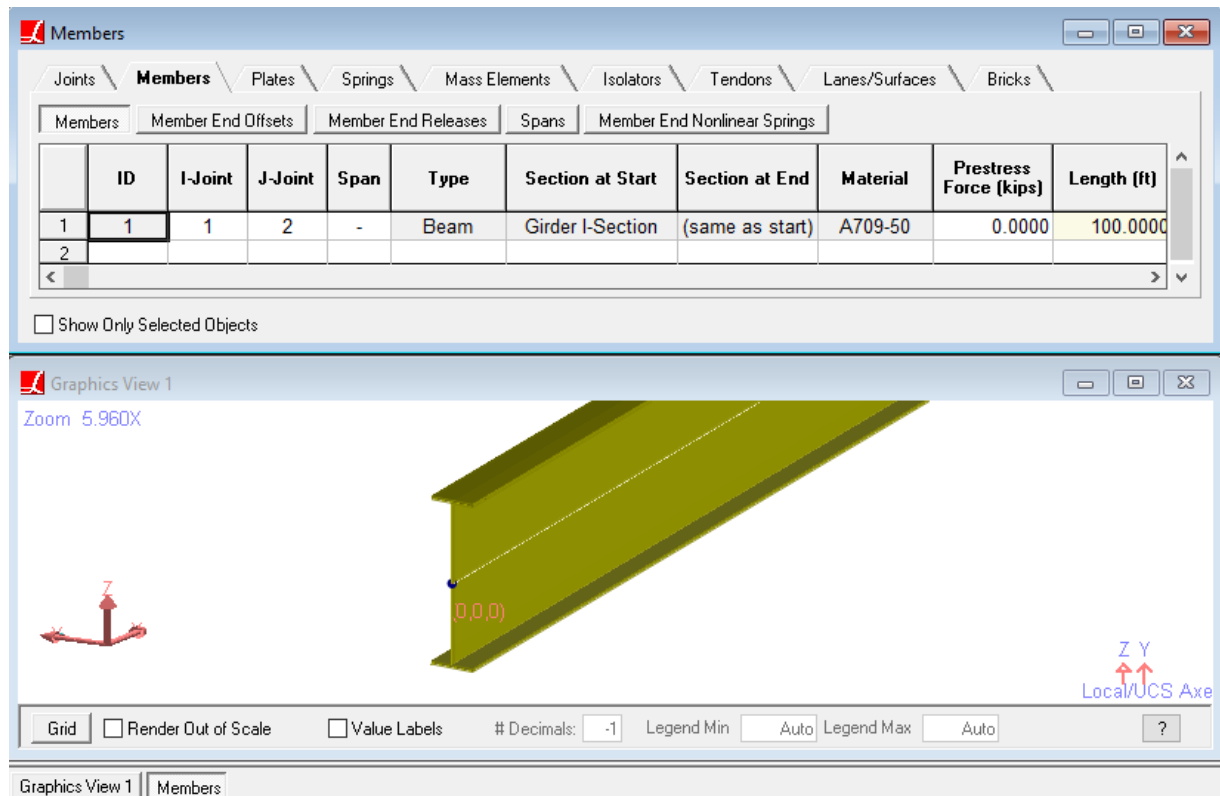
Members spreadsheet and complete rendering of the model
