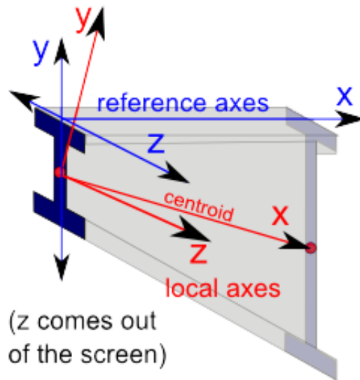
Member Reference and Local Axes - Nonprismatic Variation
