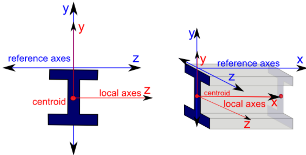
Member Reference and Local Axes - With A Centroid Offset
