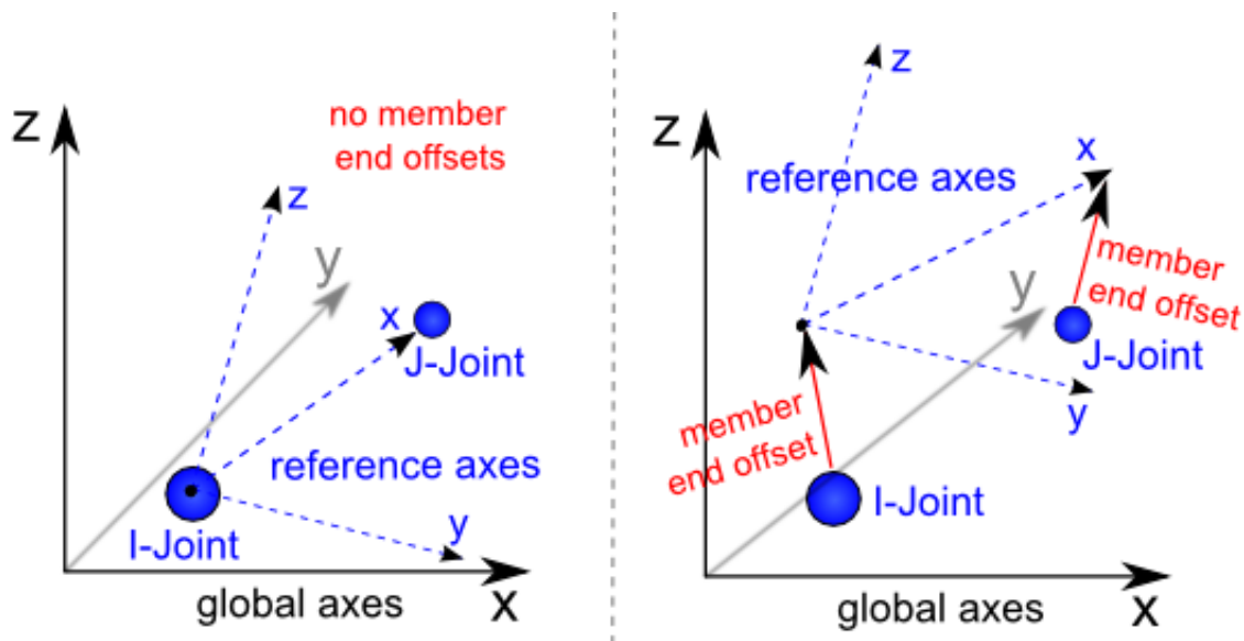
Member Reference Axes - Alignment With Joints
